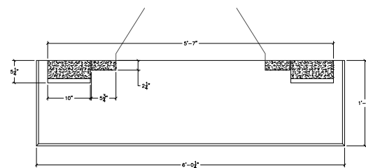
PLAN SECTION
