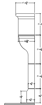
SIDE ELEVATION
