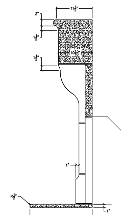
SECTION VIEW
